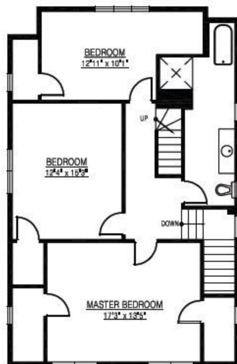
UPPER FLOOR
